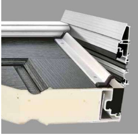
MD570 Threshold (25mm) Shown with ramp Distance from bottom of door leaf to bottom of threshold 18mm
