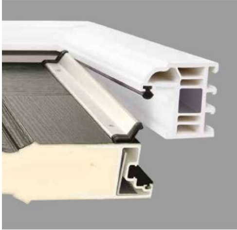
uPVC Low Frame Threshold Distance from bottom of door leaf to bottom of threshold 27mm
